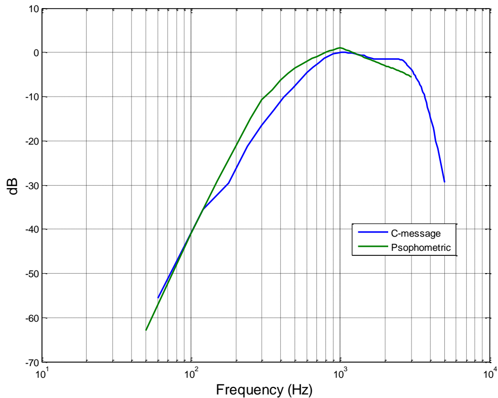
Figure 1: Comparison of CCITT Psophometric weights and C-Message weighting
